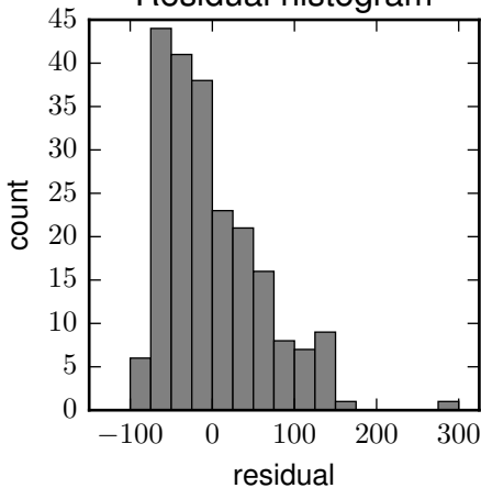
Residual histogram
