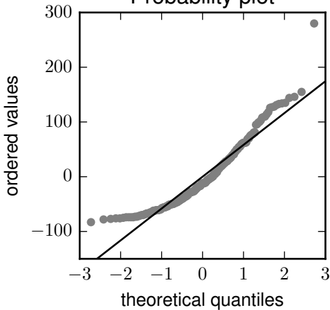
Probability plot
